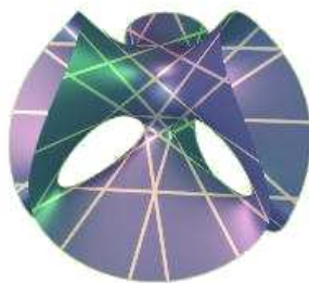
Cubic surface with 27 lines 1
