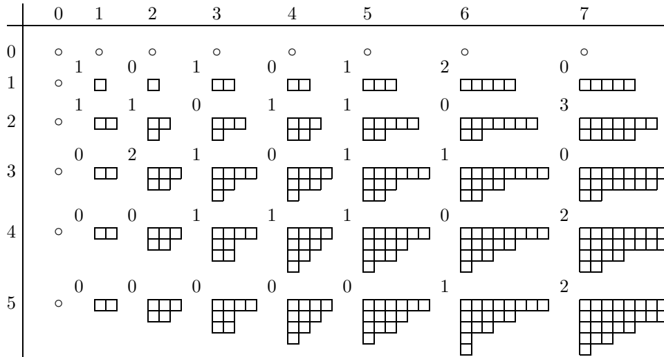
Diagram 1. Growth diagram with integral matrix and shapes (\pi(M_{[i] \times [j]}))_{i,j \in \mathbf{N}} .
