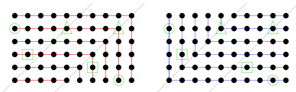
Figure 4. The action of \sigma_0^\leftarrow with ladders for e_0^- , and for \pi_r \circ e_0^- \circ \pi_r .
